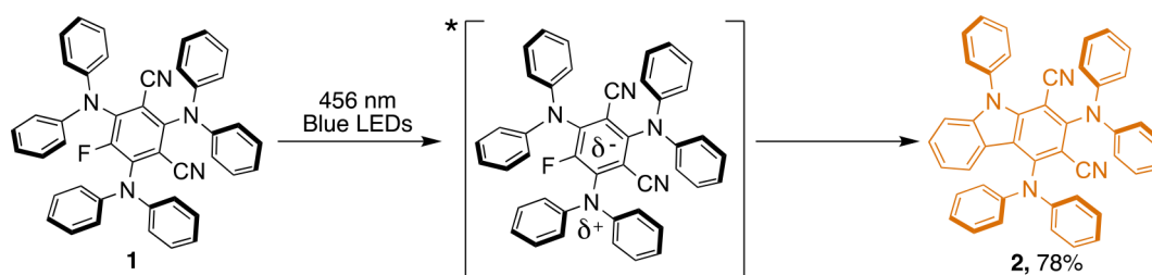
Figure 2. Charge transfer state involved in the formation of 2 by irradiation of 1 with a blue LED.
