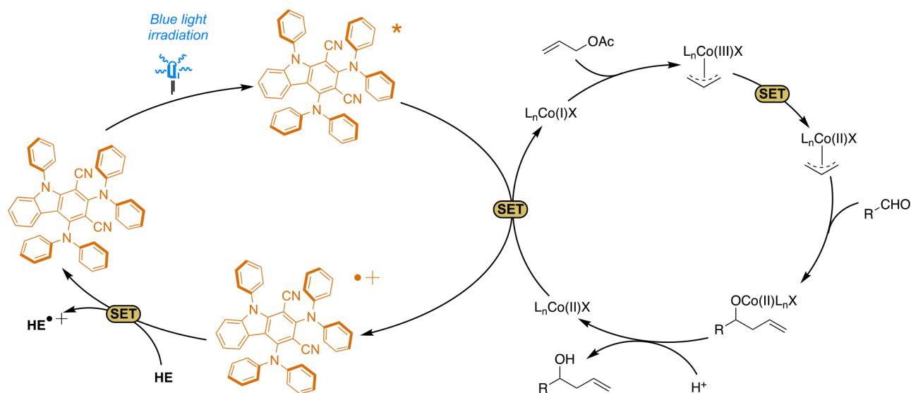
Figure 5. Suggested mechanistic picture for the reaction.
