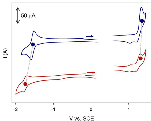
Figure 4. Cyclic voltammetry using the IUPAC convention of 1 (blue) and 2 (red) (0.5 mM) in a degassed MeCN solution containing 0.05 M tetraethylammonium hexafluorophosphate as the supporting electrolyte and ferrocene as the internal standard. Conditions: glassy carbon working electrode, Pt wire counter electrode, Ag wire quasi-reference electrode, scan rate of 1 V/s, rt. Ferrocene's peaks have been omitted for the sake of clarity.
