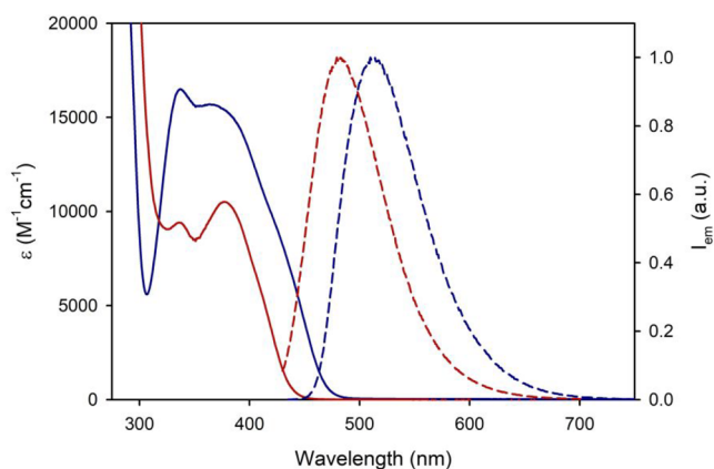
Figure 3. Absorption (solid line) and emission spectra (dashed line; \lambda_{\text{ex}} = 420 \text{ nm} ) of compounds 1 (blue) and 2 (red) in air-equilibrated THF.
