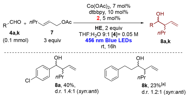
Scheme 5. Reaction of Hex-2-en-1-yl Acetate with Aromatic and Aliphatic Aldehydes
