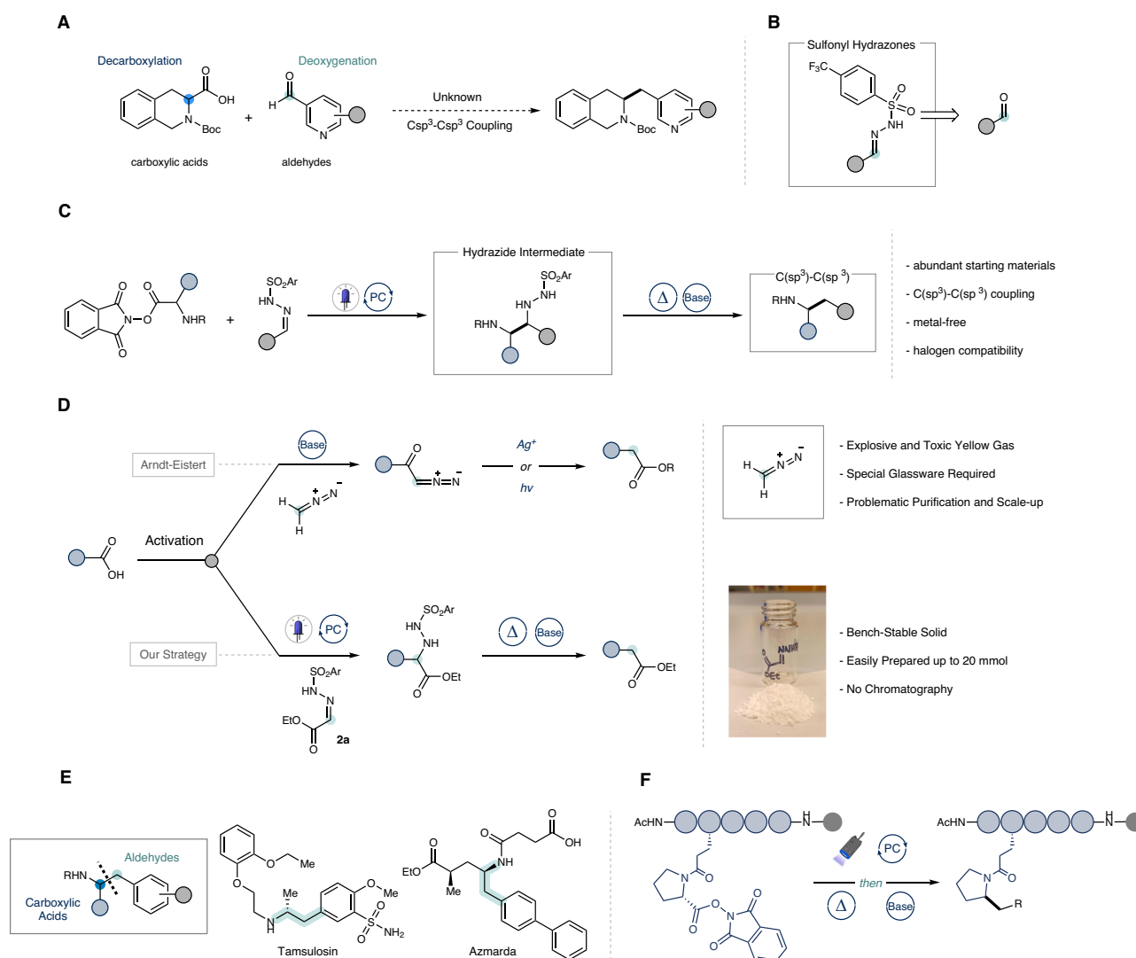
Fig. 1 | Design and applications of the cross-electrophile coupling of carboxylic acids with aldehydes. A Elusive cross-electrophile coupling between carboxylic acids and aldehydes. B Fast and scalable activation of aldehydes. C Our strategy: visible-light promoted coupling of activated carboxylic acids and sulfonyl
