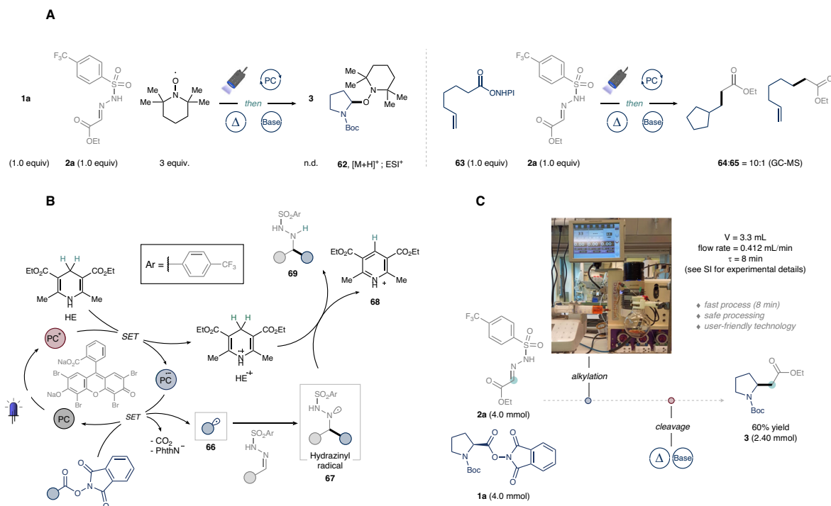
Fig. 5 | Mechanistic investigation and scale-up in flow. A Radical trapping and radical clock experiments. B Proposed mechanism. C Scale-up C1 homologation of 1a in continuous flow.
