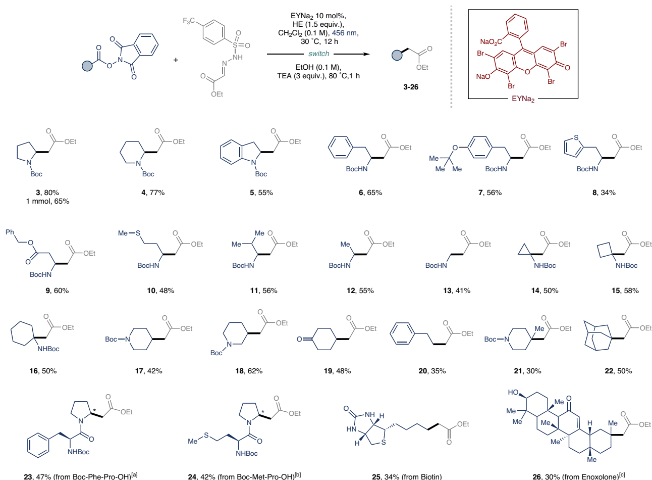
Fig. 2 | Scope of the C1 homologation. Coupling of carboxylic acid-derived redox-active esters (RAEs) with ethyl glyoxalate-derived 4-trifluoromethylphenyl sulfonyl hydrazones 2a . Reaction conditions: redox active ester (0.3 mmol, 1 equiv.), 2a (1
